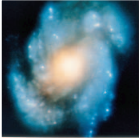
The Hubble Space Telescope is above Earth's atmosphere and forms clearer images of objects in space.
