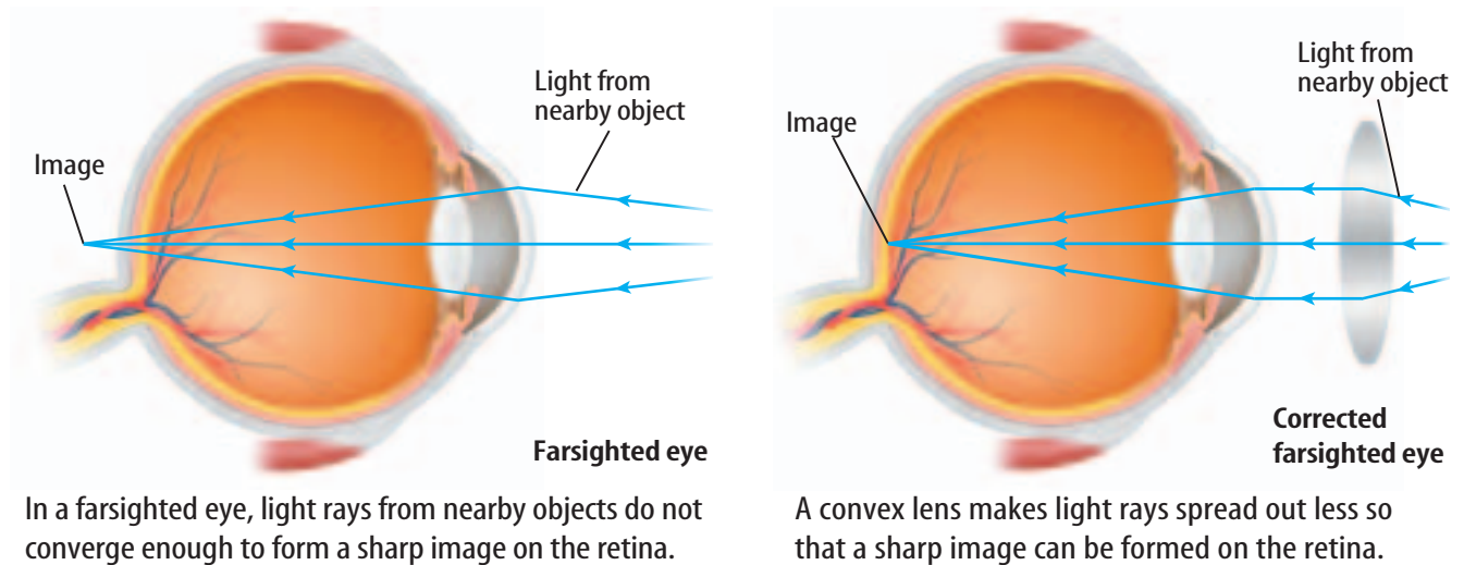
Figure 14 Farsightedness can be corrected by a convex lens.
