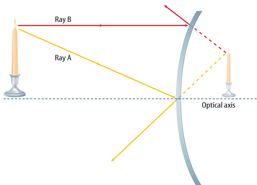
Figure 8 A convex mirror forms a reduced, upright, virtual image.
