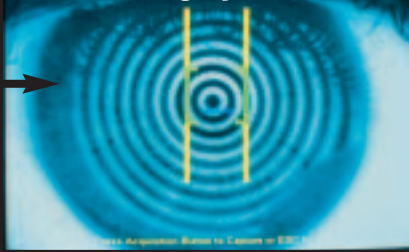
Measuring the eye for laser surgery
