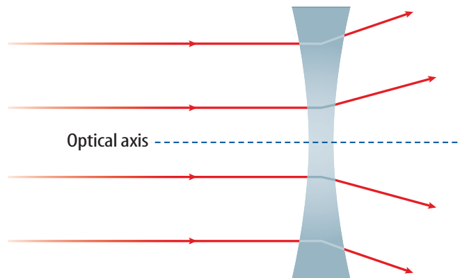
Figure 11 A concave lens refracts light rays so they spread out.
