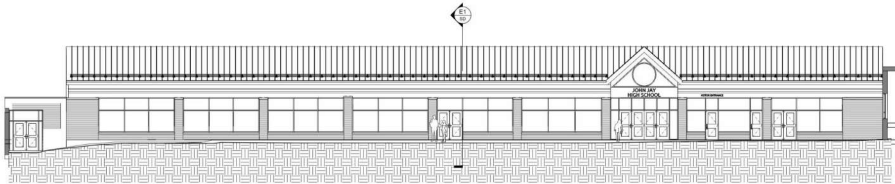
SOUTH ELEVATION
